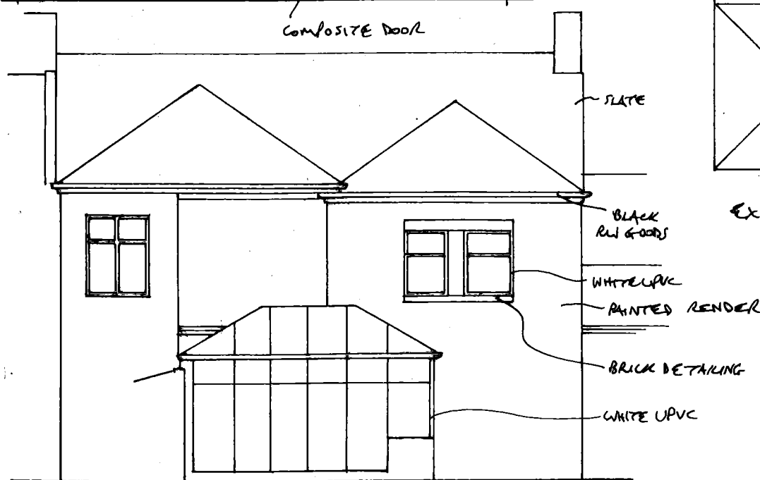
EXISTING REAR 1:100
